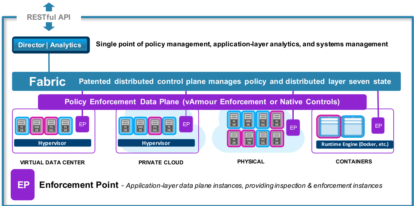
Figure 1. vArmour system architecture 1
